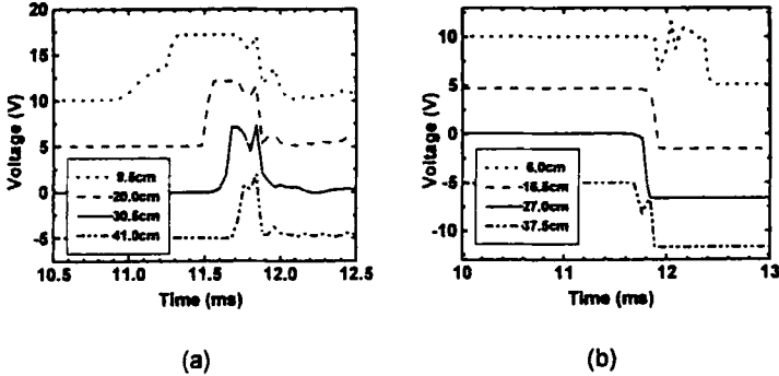
Fig. 6 (a) Optoelectronic Triode Curves, (b) Strain Gauge Curves of Test No. 1.
